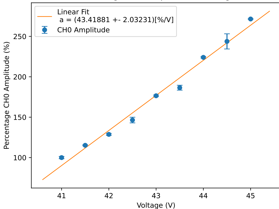
Percentage CH0 Amplitude vs Voltage
