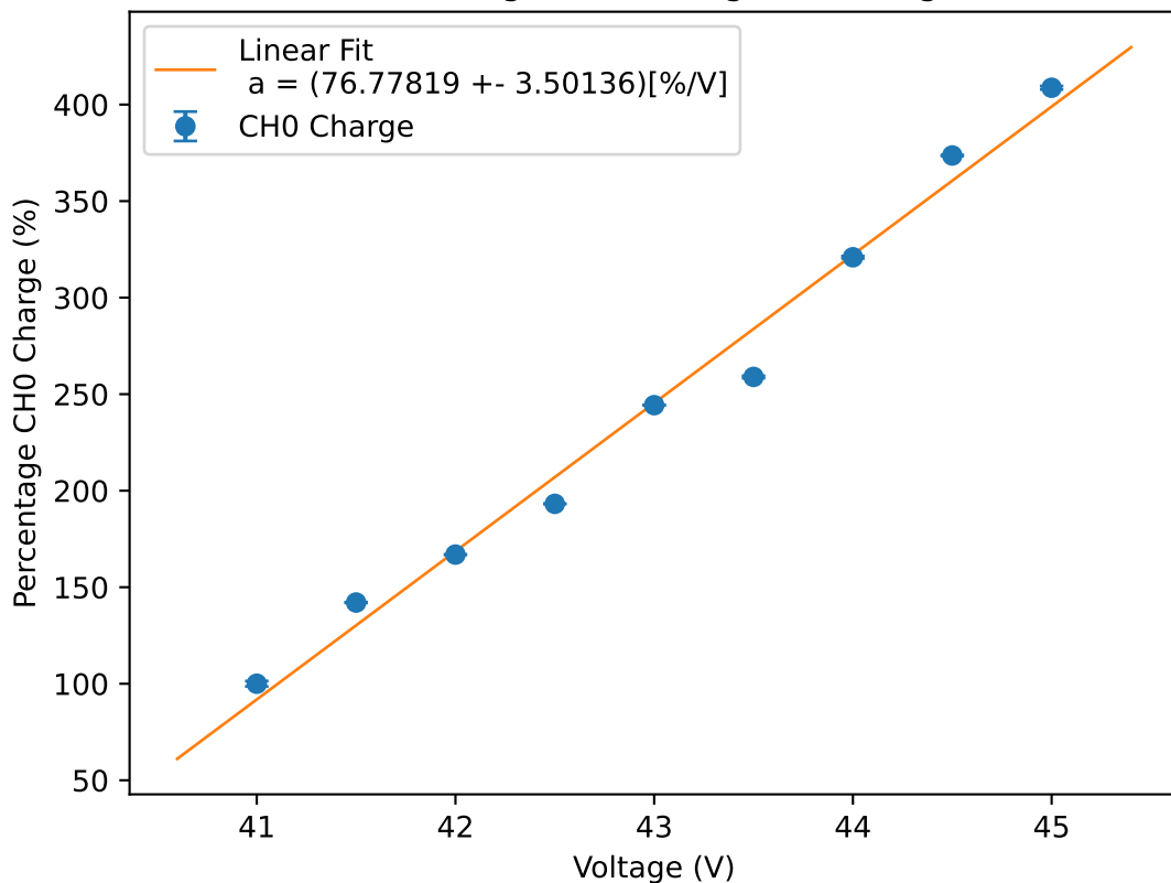
Percentage CH0 Charge vs Voltage
