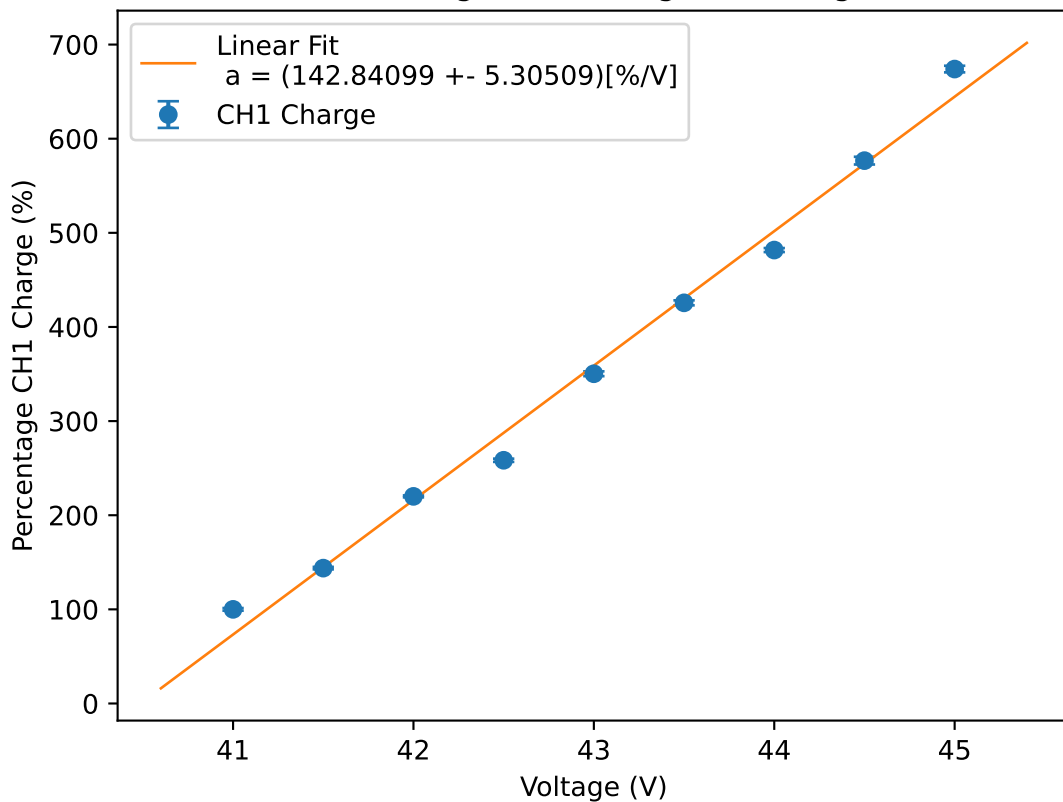
Percentage CH1 Charge vs Voltage
