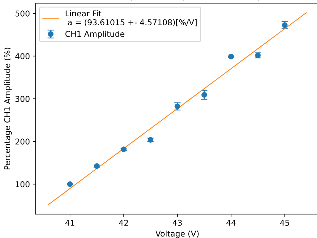
Percentage CH1 Amplitude vs Voltage
